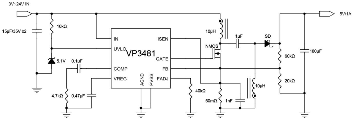
Figure8 VP3481 Typical SEPIC Application
