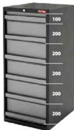
HT-1261 (47-01) 547W x 600D x 1200H mm
