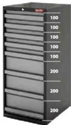
HT-1281 (47-04) 547W x 600D x 1200H mm
