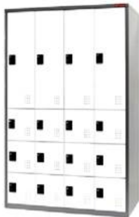
FC1M-416 (30-08) 1182W x 510D x 1800H mm
