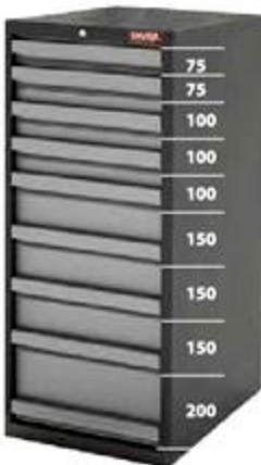
HT-1291 (47-05) 547W x 600D x 1200H mm
